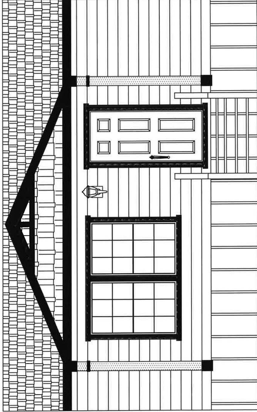
EXTERIOR ELEVATION 8A
