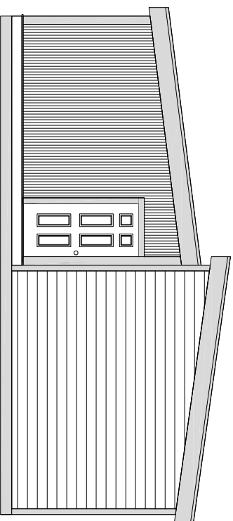
Left Elevation
